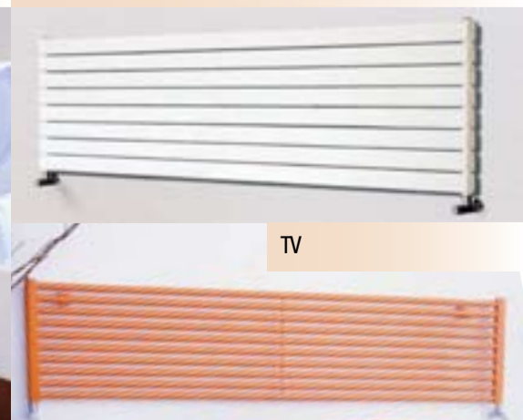
SVD Double
